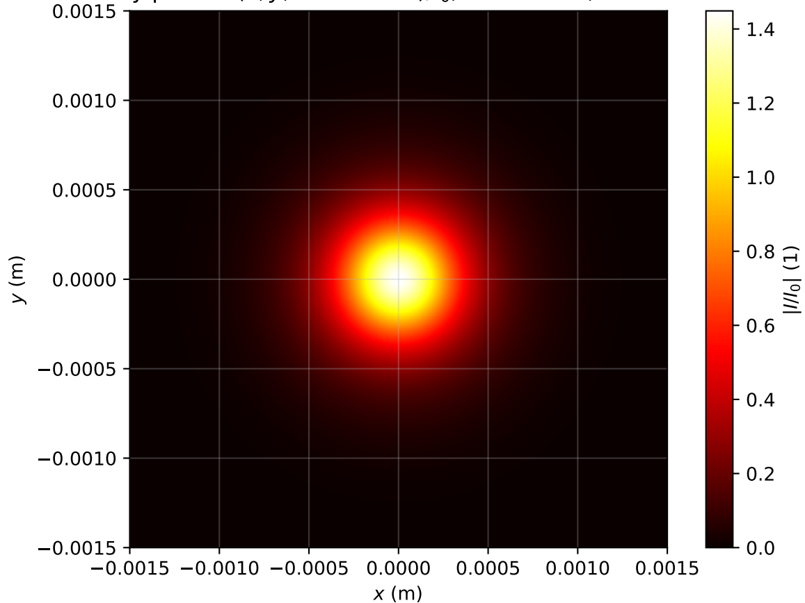
Intensity profile I(x, y, z = 1.115m)/I_0 , P_{in}=0.9P_{cr} , artificial time
